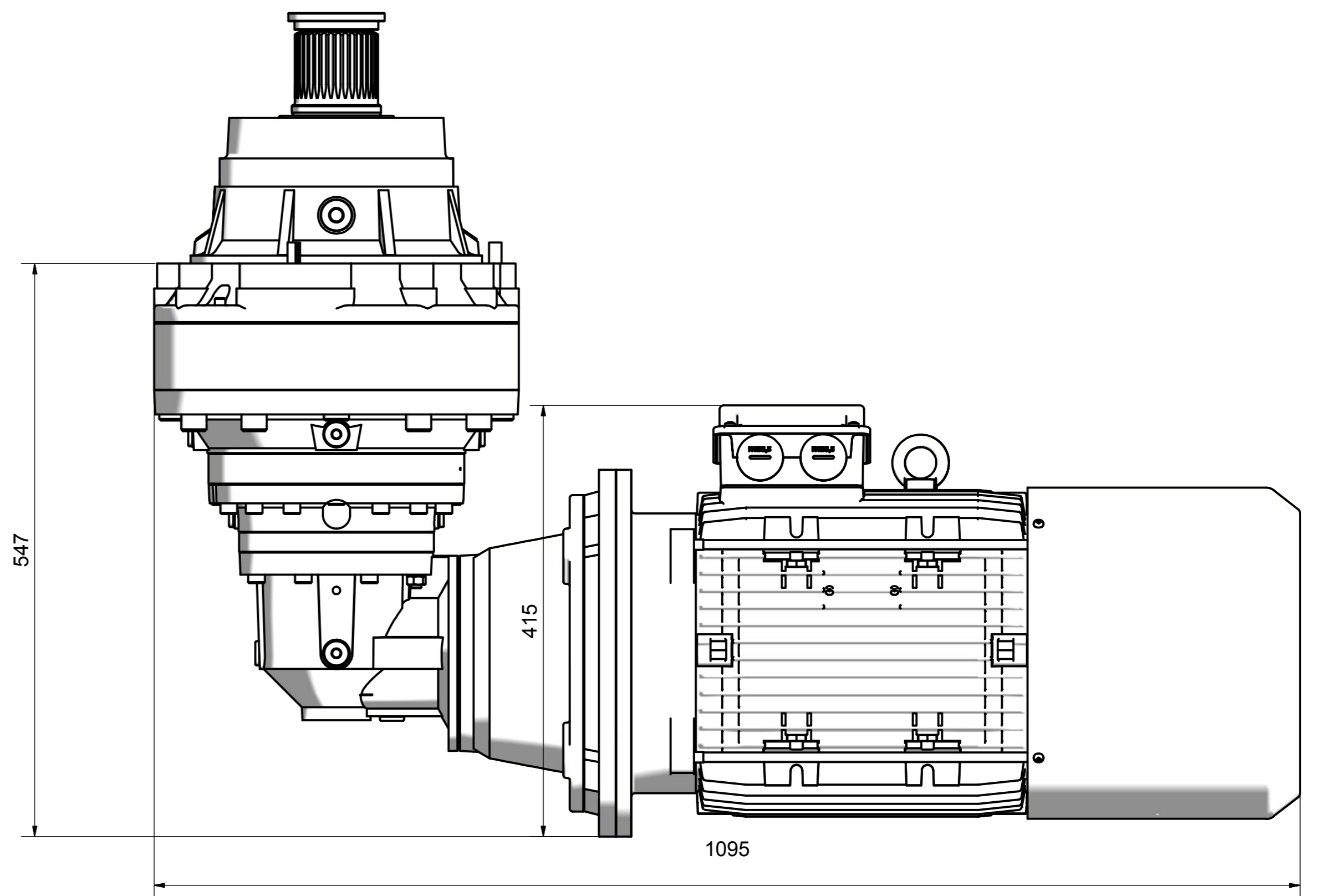
Alternative Angled Drive
